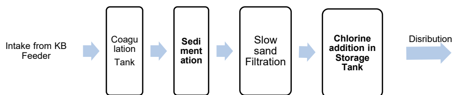
Figure 4.3. Treatment process at MUET water Treatment Plant
